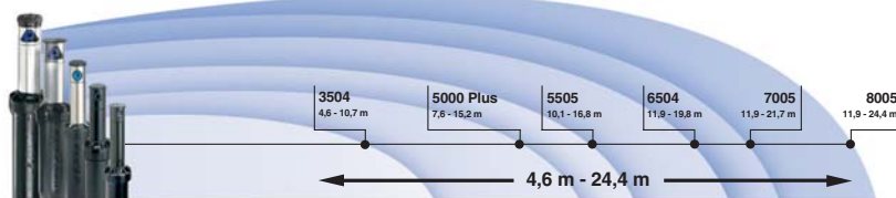
Rain Curtain™ Nozzle Buses Rain Curtain™
